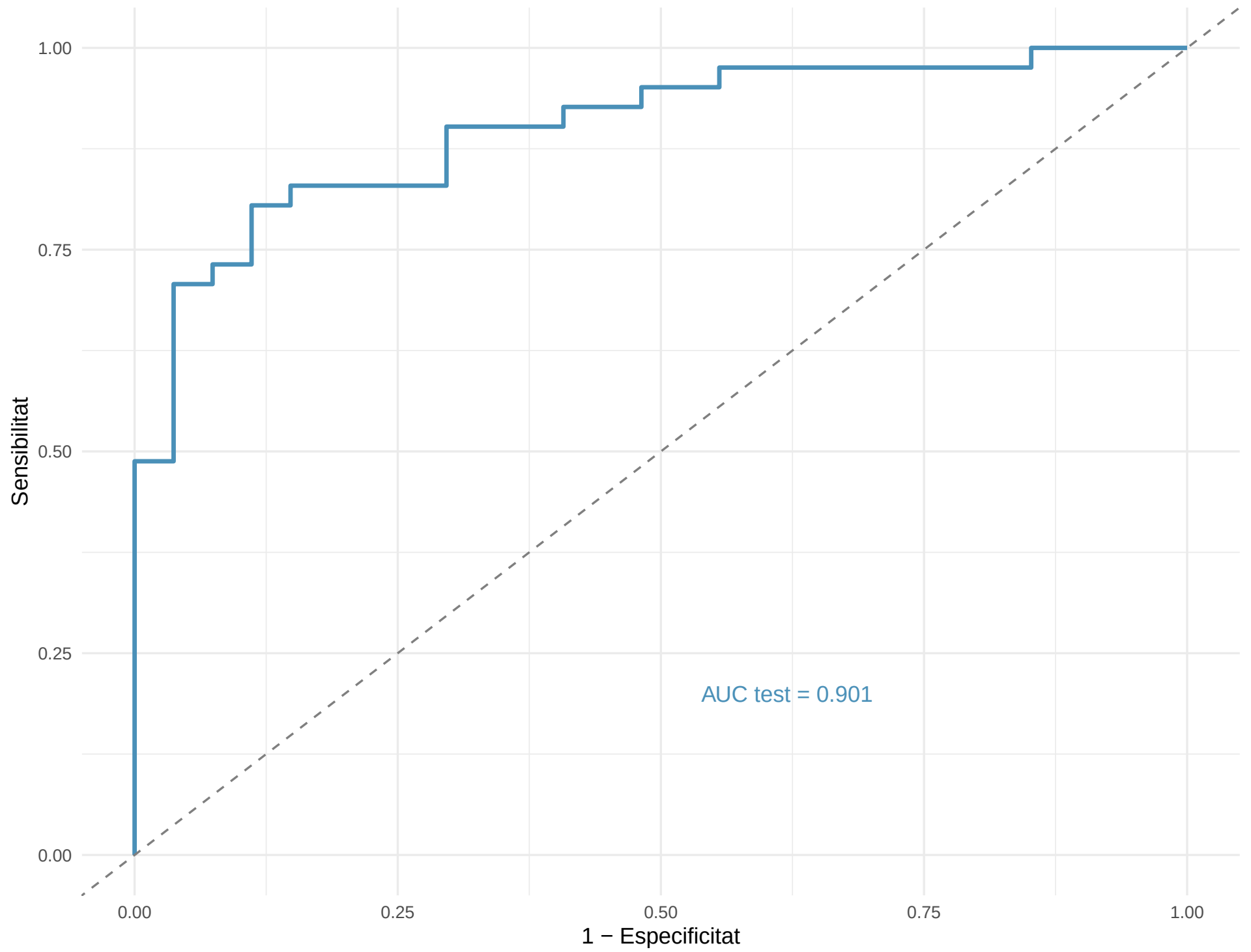
Corba ROC — XGBoost (test)
